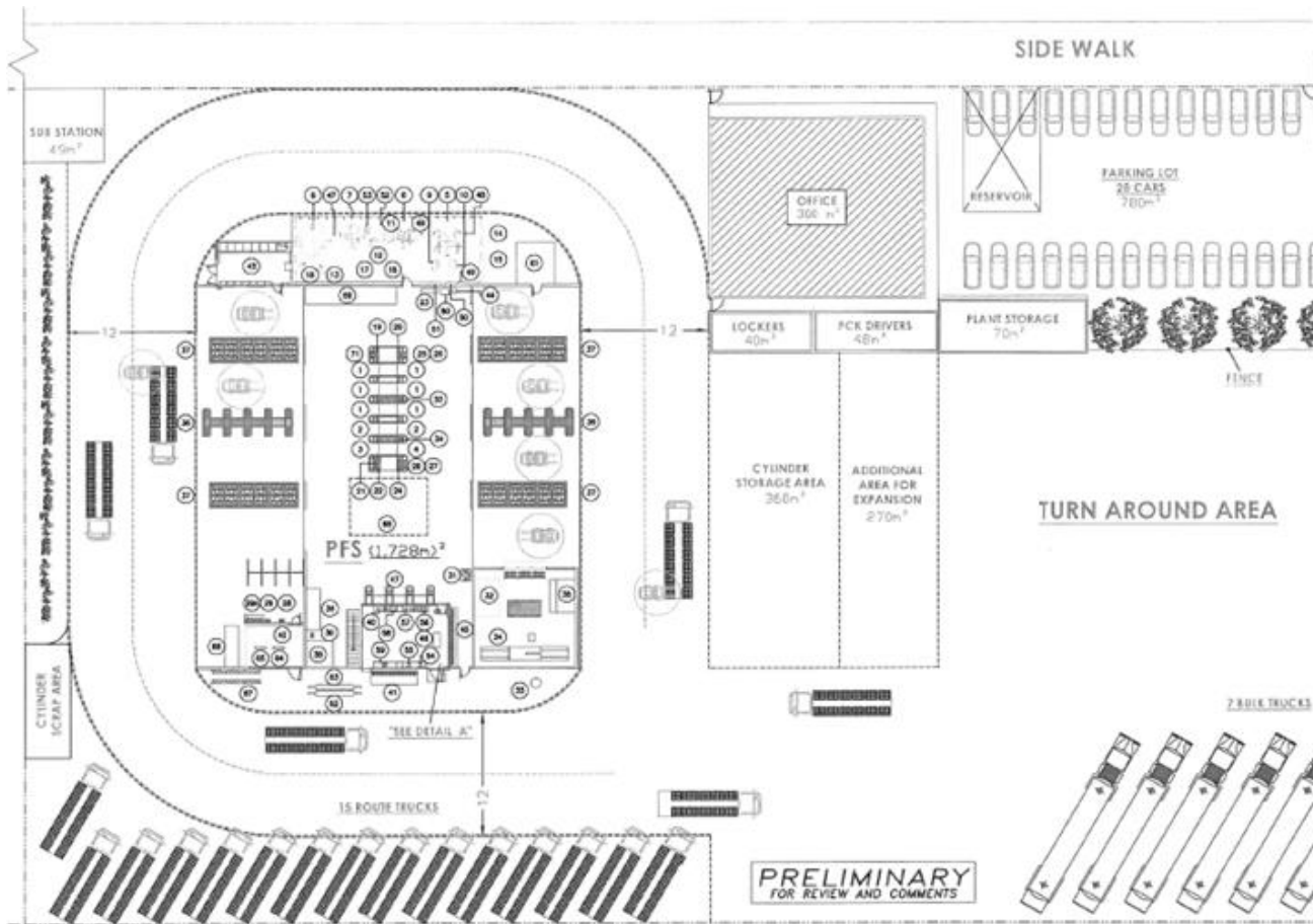
Preliminary layout
